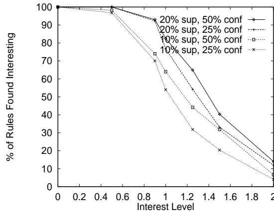
Figure 8: Interest Measure
