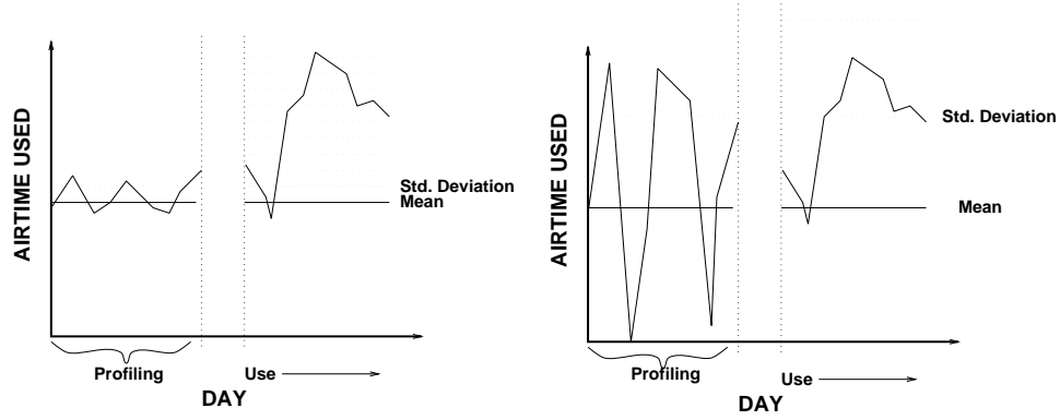
Figure 6. Using mean and standard deviation in profiling.
