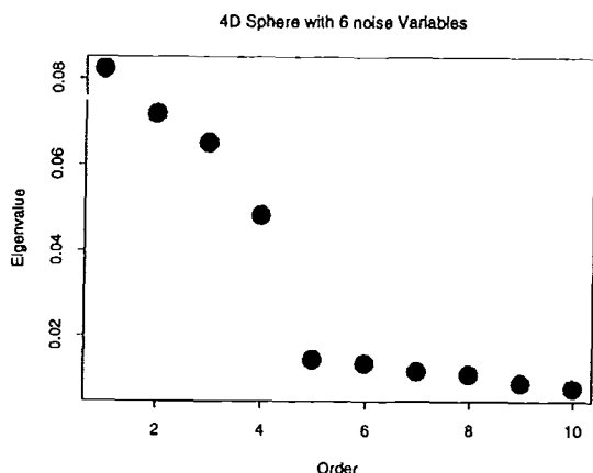
Figure 4: The eigenvalues of the average between matrix for the 4D sphere + 6 noise variable problem. Using these first four dimensions followed by our DANN nearest neighbor routine, we get better performance than 5NN in the real 4D subspace.
